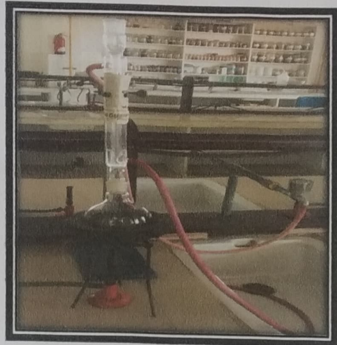
Soxhlet apparatus
